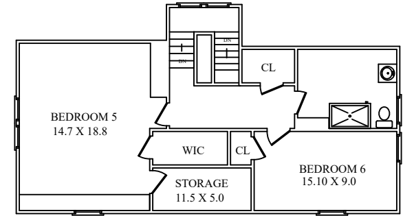
THIRD LEVEL
