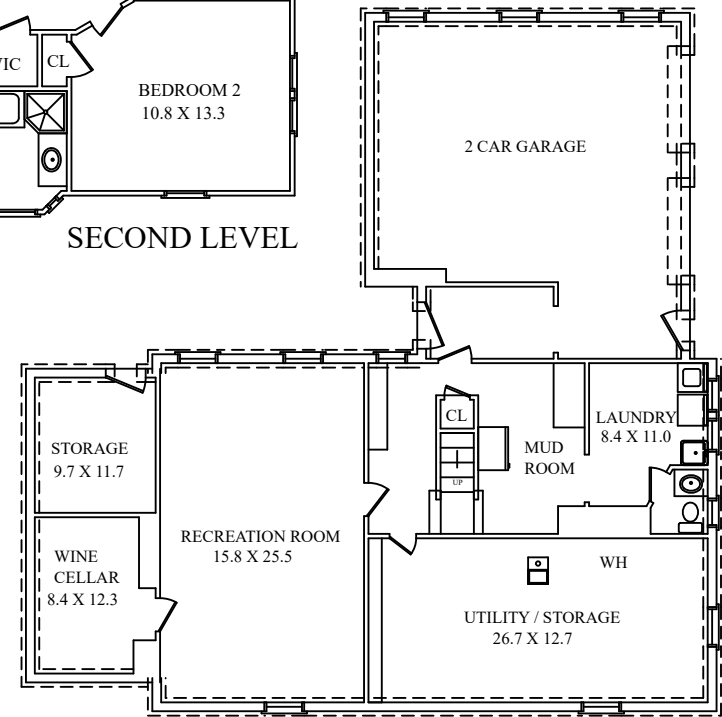
LOWER LEVEL
