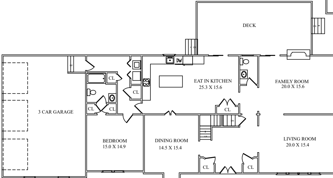
FIRST LEVEL
