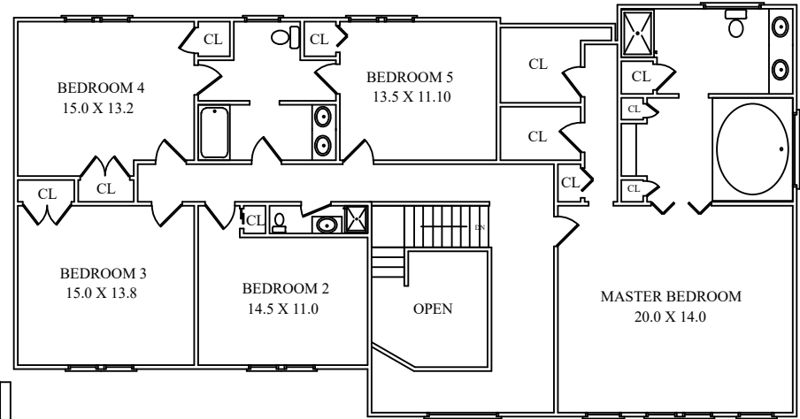
SECOND LEVEL
