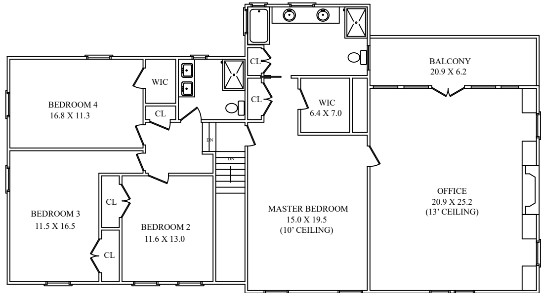
SECOND LEVEL
