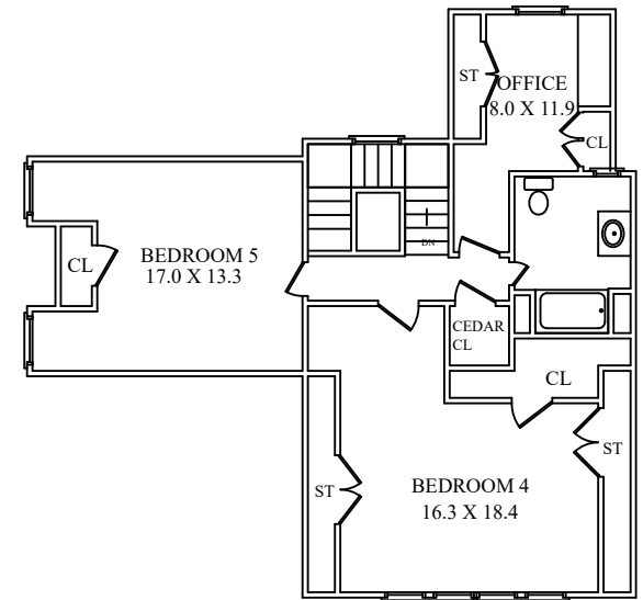
THIRD LEVEL
