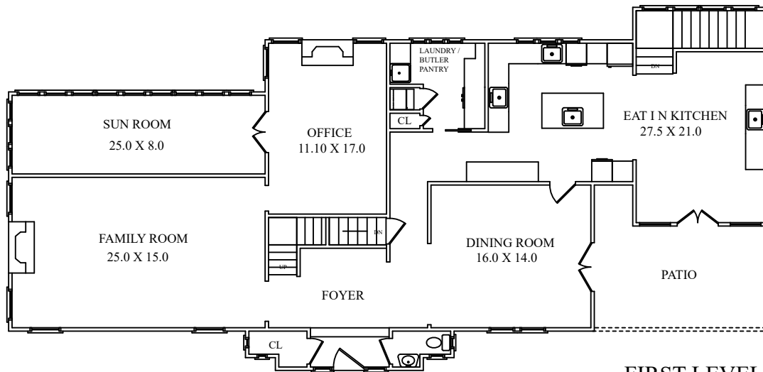
FIRST LEVEL
