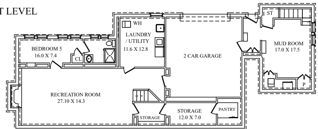
LOWER LEVEL
