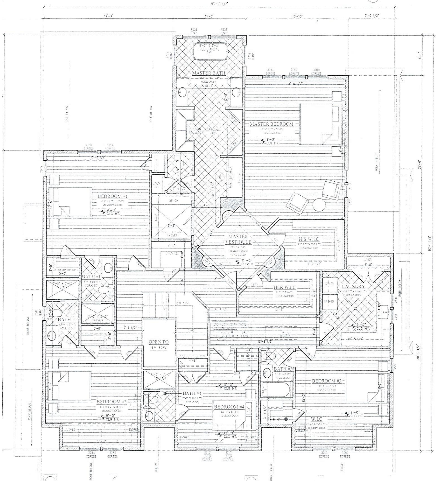
4 SECOND FLOOR PLAN
