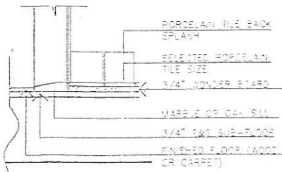
1 CERAMIC TILE DETAIL
