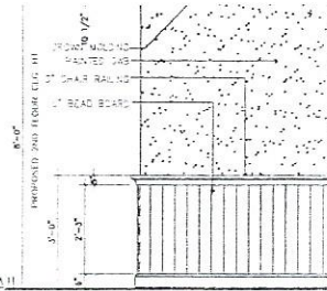
2 OPTIONAL BEADBOARD PANEL DETAIL
