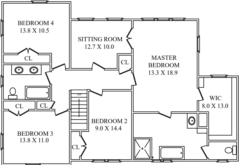
SECOND LEVEL
