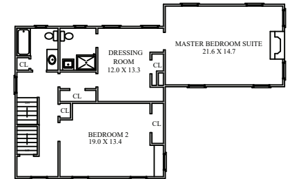
COTTAGE SECOND LEVEL
