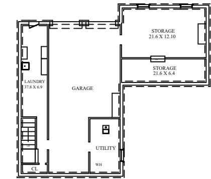
COTTAGE LOWER LEVEL
