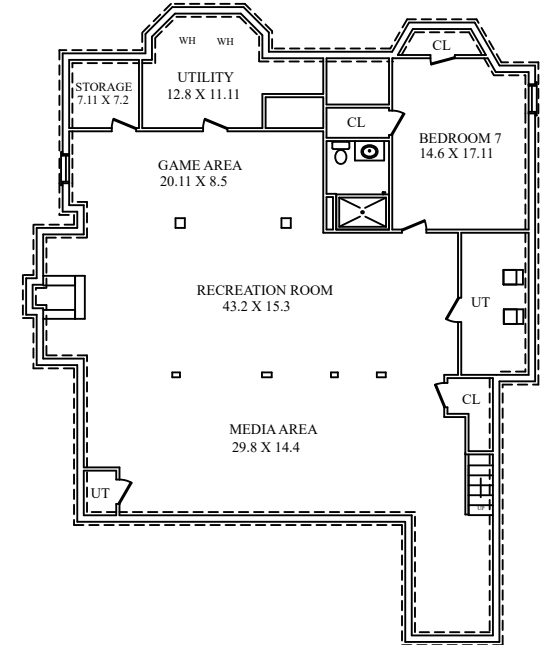
LOWER LEVEL
