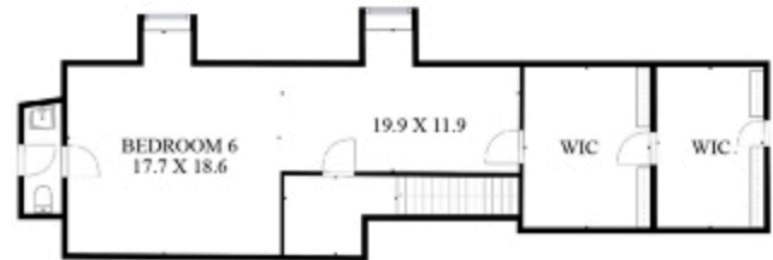
THIRD FLOOR
