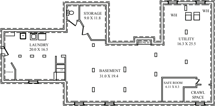
LOWER LEVEL
