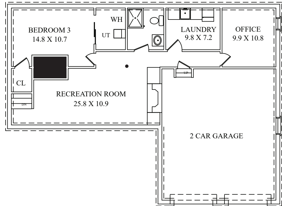
LOWER LEVEL
