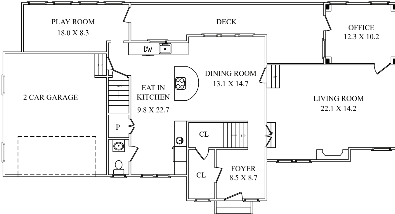
FIRST LEVEL
