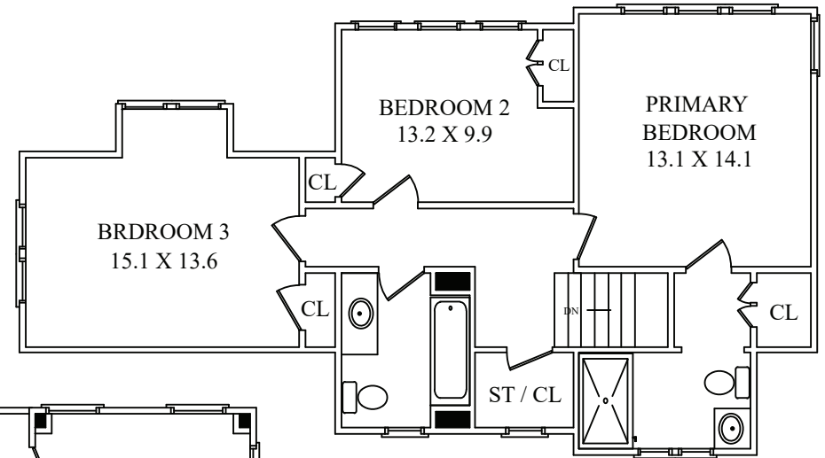
SECOND LEVEL
