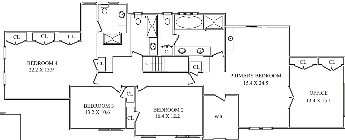
SECOND LEVEL
