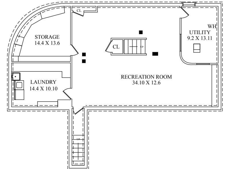
LOWER LEVEL
