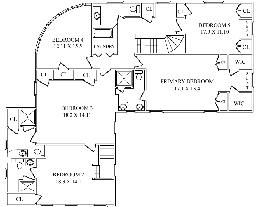
SECOND LEVEL
